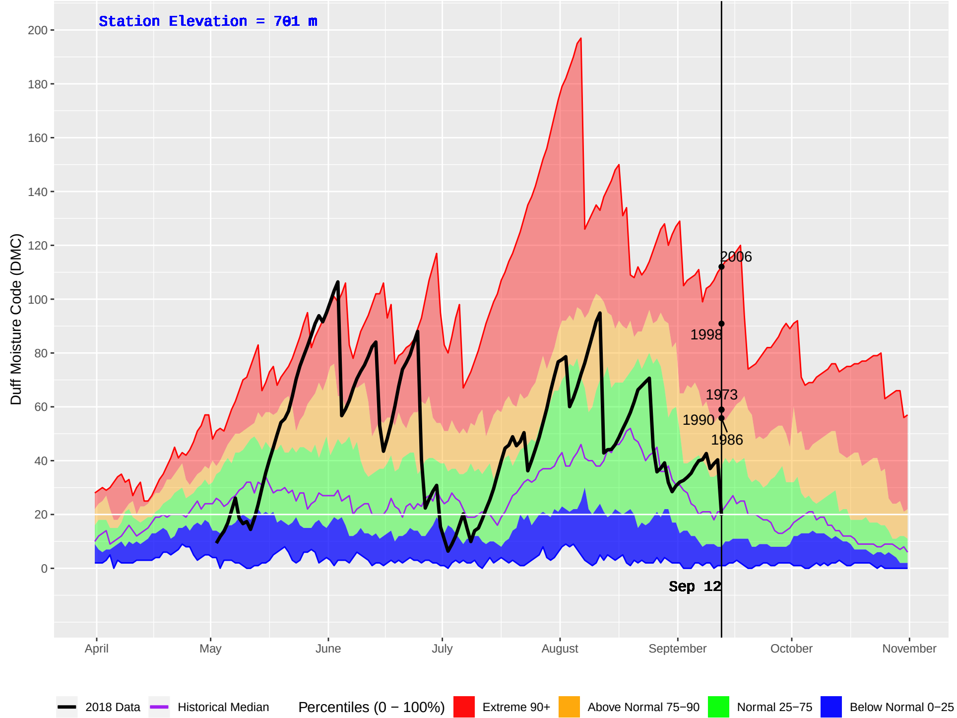
HORSEFLY (230) : Historical (1971–2016) and Current (2018) Daily Duff Moisture Code (DMC)
