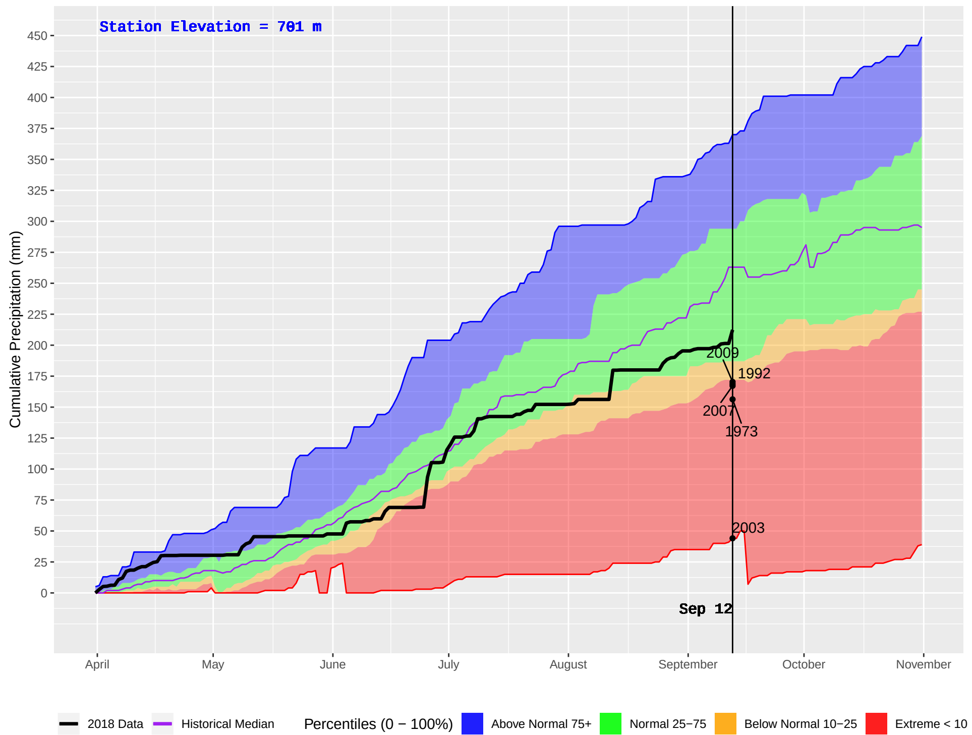
HORSEFLY (230) : Historical (1971–2016) and Current (2018) Daily Cumulative Precipitation
