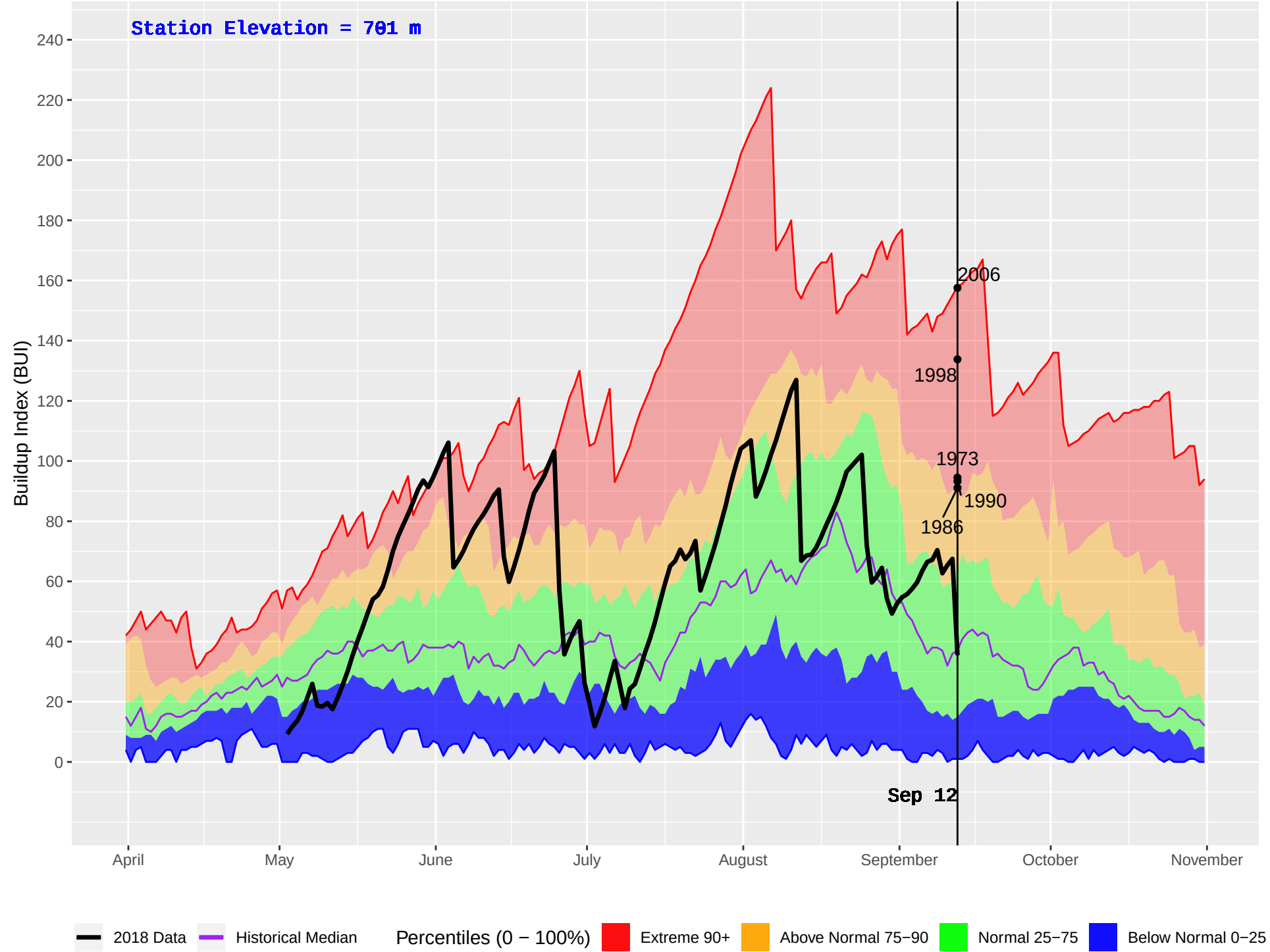
HORSEFLY (230) : Historical (1971–2016) and Current (2018) Daily Buildup Index (BUI)
