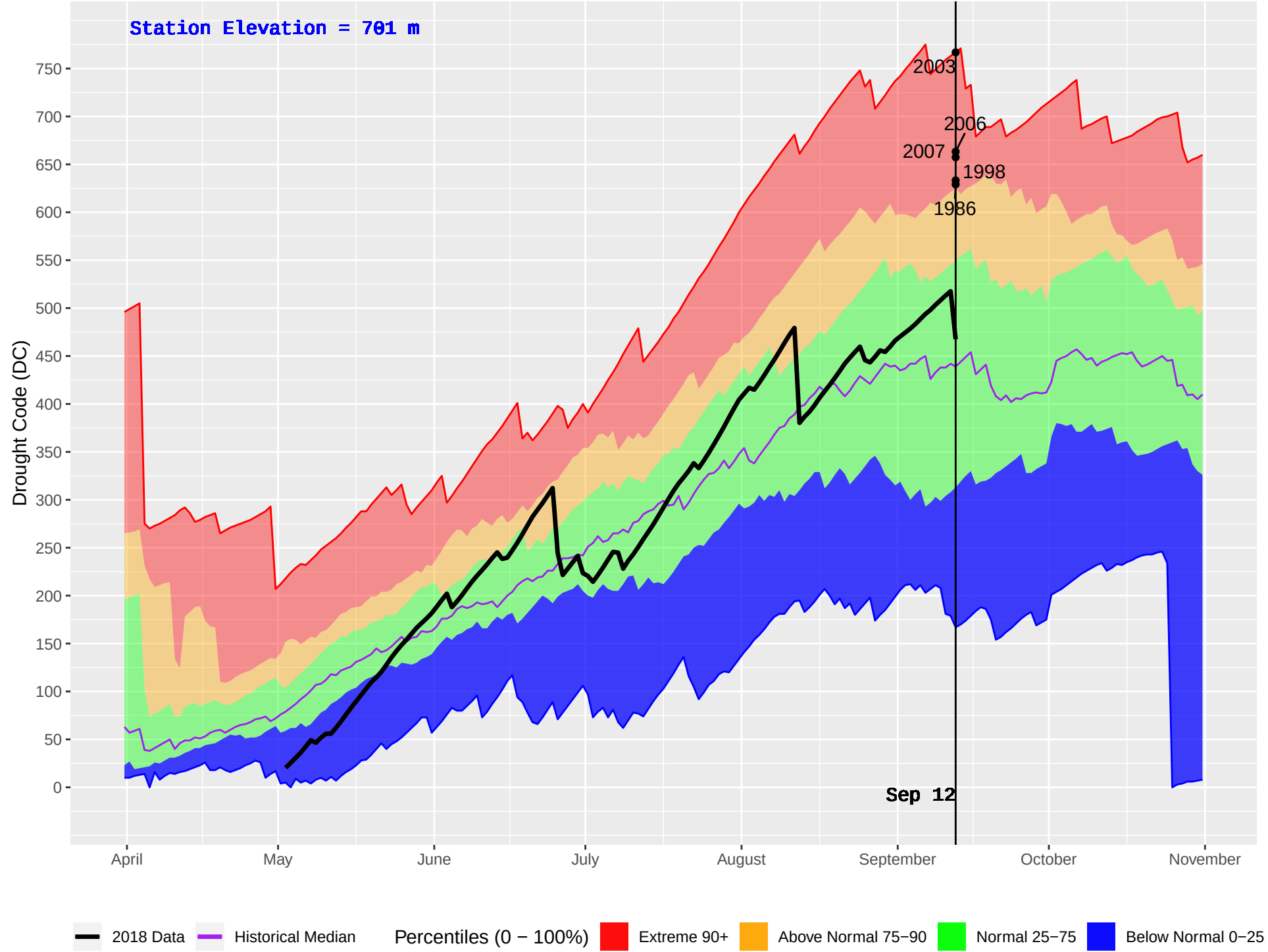
HORSEFLY (230) : Historical (1971–2016) and Current (2018) Daily Drought Code (DC)
